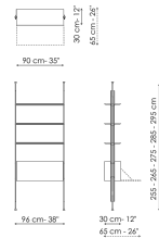
Ceiling fixing 1 module Width: 96cm Depth: 30cm Height: 255-265-275-285-295cm
