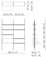
Ceiling fixing 2 modules Width: 188cm Depth: 30cm Height: 255-265-275-285-295cm
