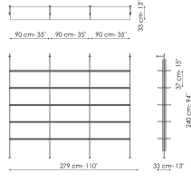
Wall fixing 3 modules Width: 280cm Depth: 33cm Height: 240cm
