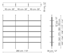
Ceiling fixing 3 modules Width: 280cm Depth: 30cm Height: 255-265-275-285-295cm
