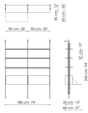
Wall fixing 2 modules Width: 188cm Depth: 33cm Height: 240cm
