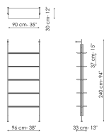
Wall fixing 1 module Width: 96cm Depth: 33cm Height: 240cm
