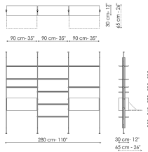
Ceiling fixing 3 modules Width: 280cm Depth: 30cm Height: 255-265-275-285-295cm
