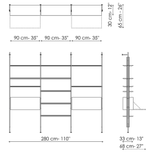
Wall fixing 3 modules Width: 280cm Depth: 33cm Height: 240cm
