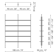
Ceiling fixing 2 modules Width: 188cm Depth: 30cm Height: 255-265-275-285-295cm
